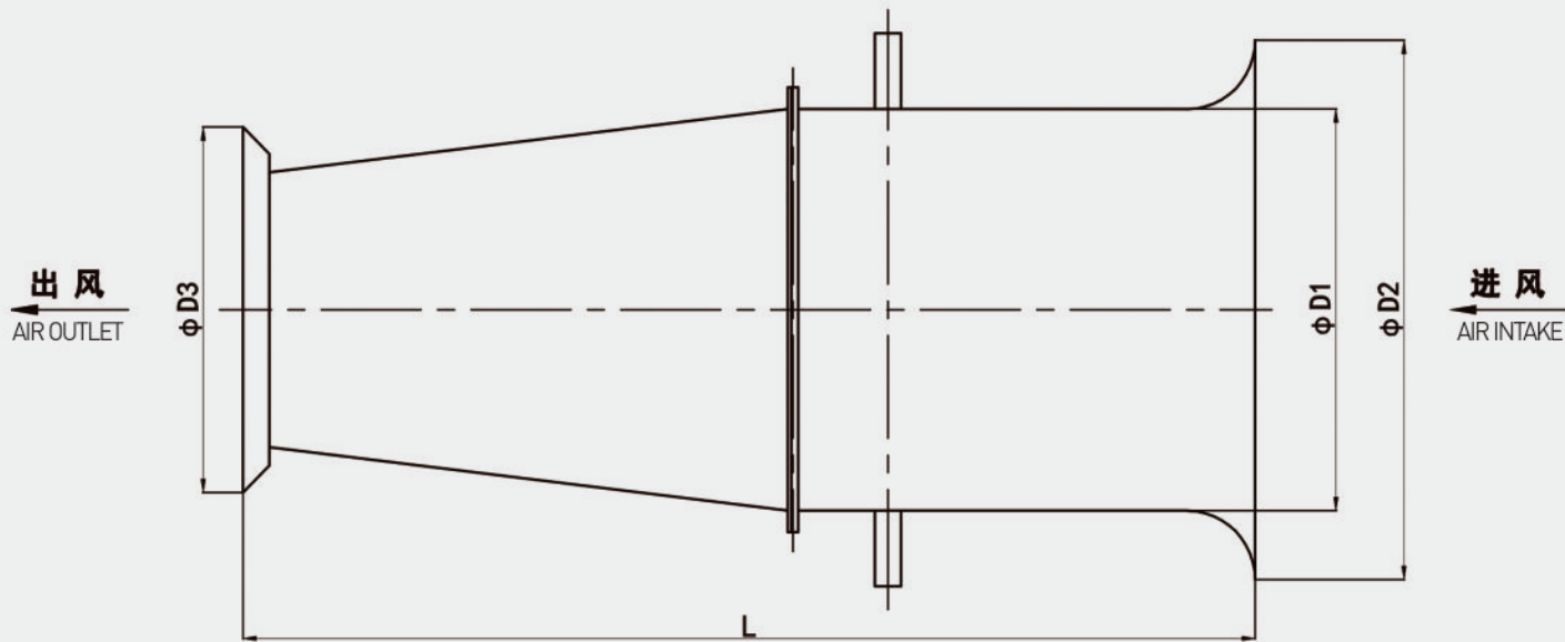
射流喷雾风机外形尺寸图 FIGURE SIZE OF SPRAY FAN
